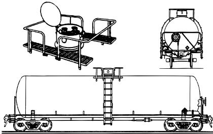
Pressure Tank Car Compressed Liquefied Gases (Closed Dome Only on top) (117)
